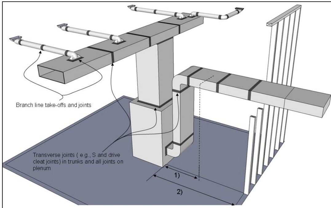
Figure 1: Duct Sealing Requirements Forming Part of 4.7.2.3 (a) (ii)
